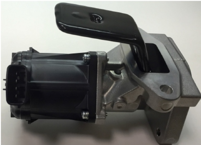
Mechanical EGR Tool shown properly positioned into the side opening of EGR valve.
