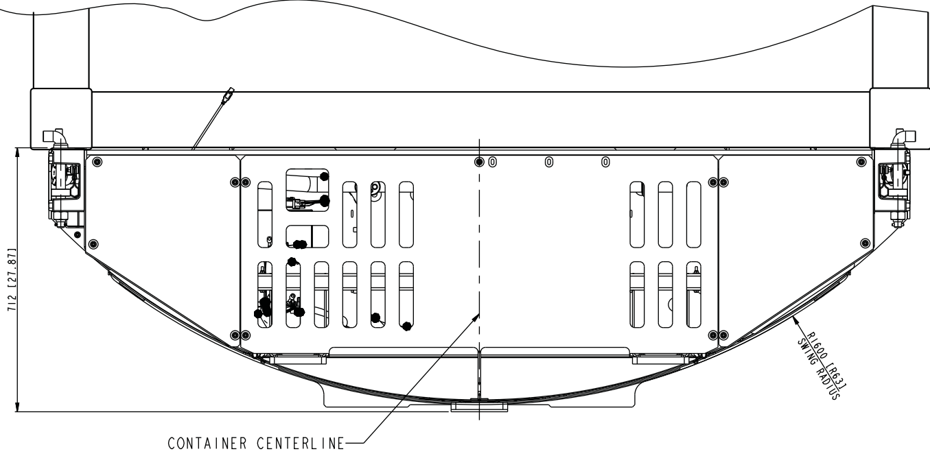
BOTTOM VIEW
